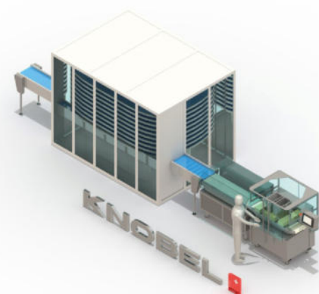
Step 1: KCM Alpha Compact with Vibrationtable and Cooling-Spiral
